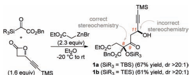
Scheme 1. Three-Component Coupling
