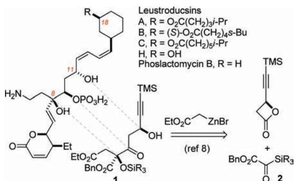
Figure 1. Leustroductsin B and related compounds.
